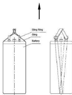
OPZV Battery Hoisting Layout
